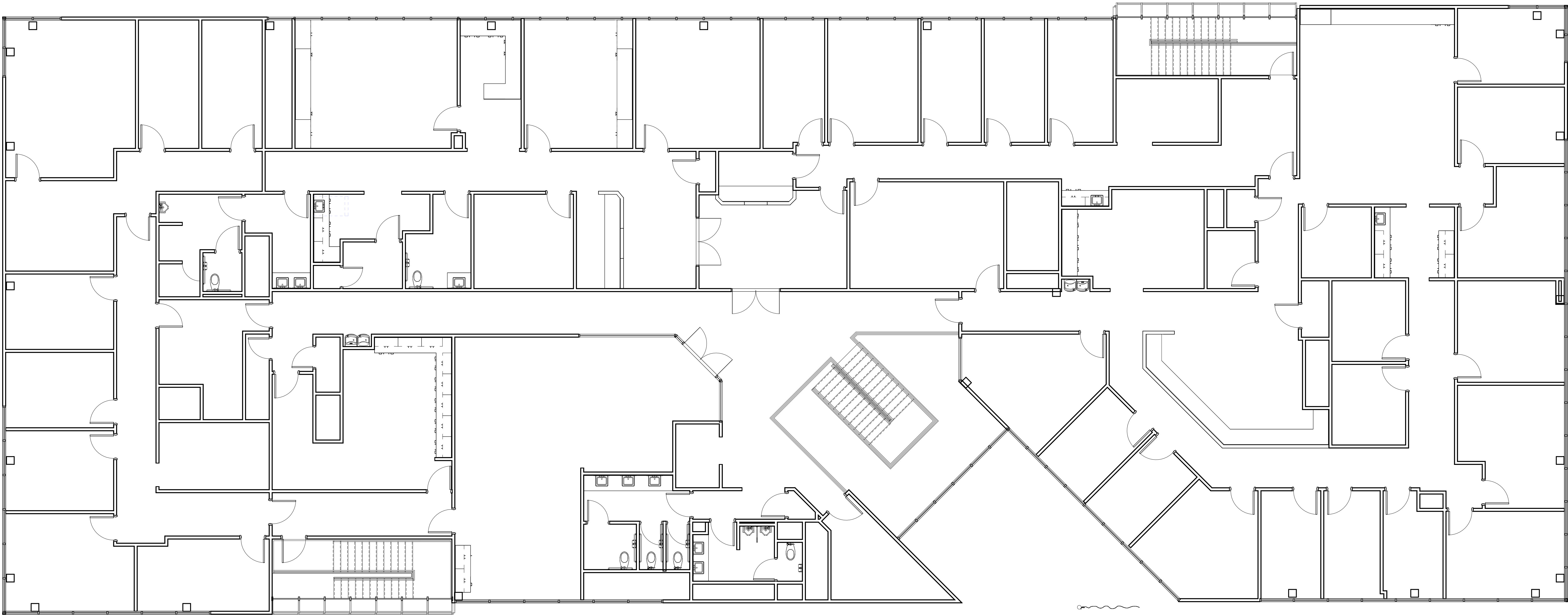
1 EXISTING FLOOR PLAN - LEVEL 2 3/16" = 1'-0"
