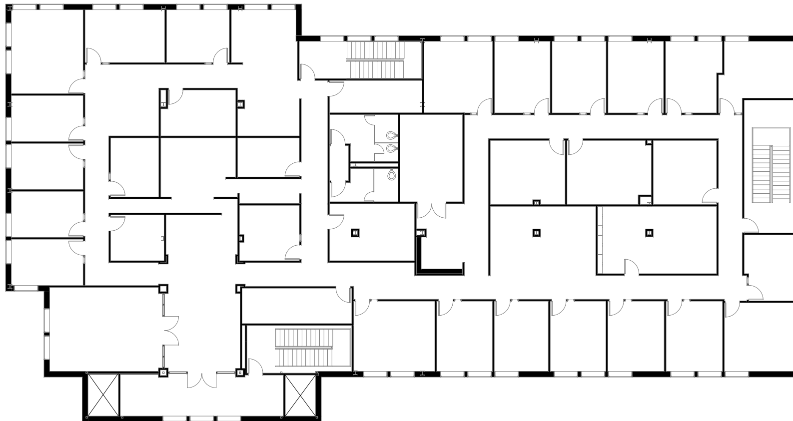
① LEVEL 4 LEASE PLAN 1" = 20'-0"
