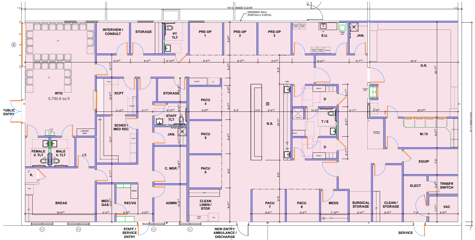
Suite 100 A ~6,844 SF
