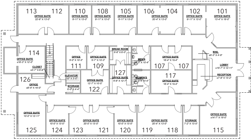
LEVEL 1 FLOOR PLAN 1/8" = 1'-0"
