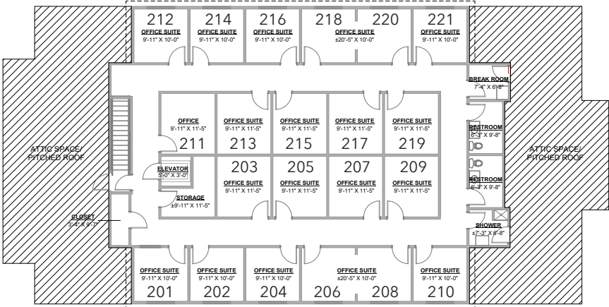
LEVEL 2 FLOOR PLAN 1/8" = 1'-0"
