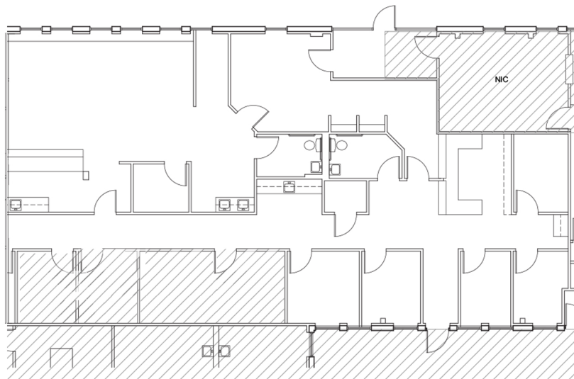
SUITE 550 FLOOR PLAN
